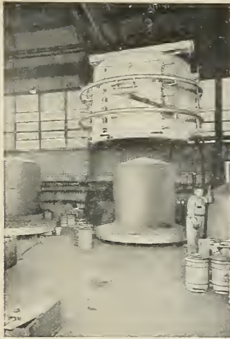
The 72-inch dia. hydrogen atmosphere furnace being lowered over a loaded furnace bell. Detroit plant.
