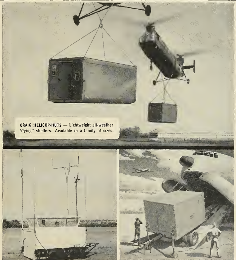
OBSERVATION-DOME SHELTER with 4-wheel dolly for air traffic control and other operation.
