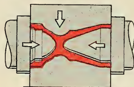
Movement of the three elements in the split-die process.
