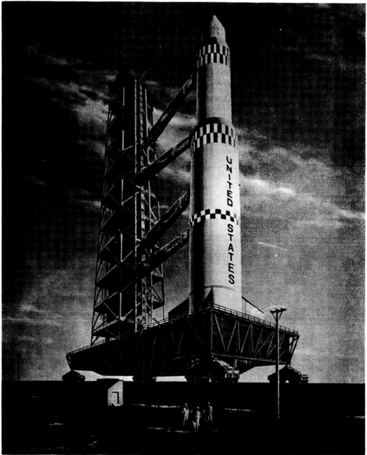
FIGURE 14. SATURN MOBILE LAUNCHER/TRANSPORTER-RAIL CONCEPT
