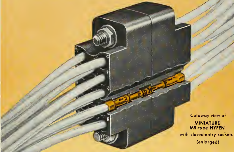
15 contact, multi-purpose connector. Mates with, or re- places existing solder con- nectors.
