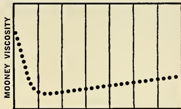
MOONEY SCORCH CURVE for FLUOREL 2141
