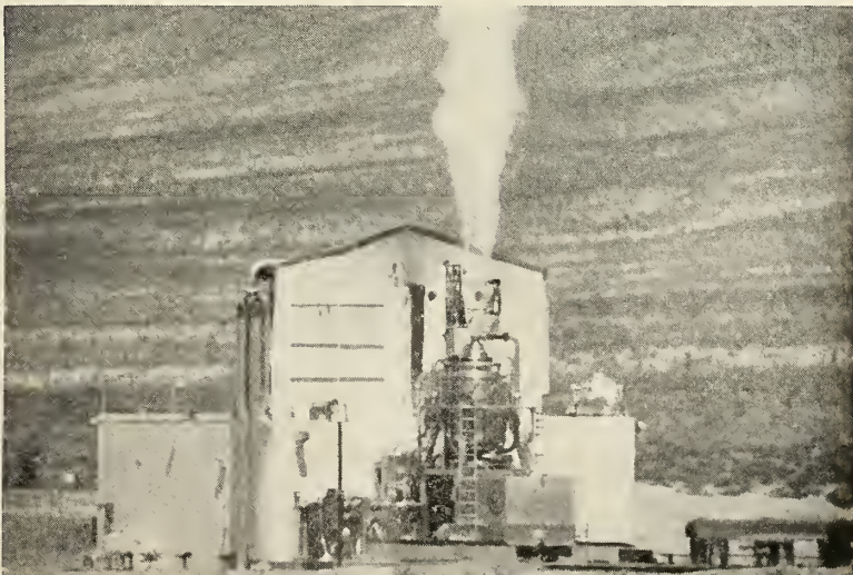
FIRST NUCLEAR rocket spouts hydrogen in test of AEC's Kiwi-A at Nevada test site last summer. Two more tests are scheduled this summer.
