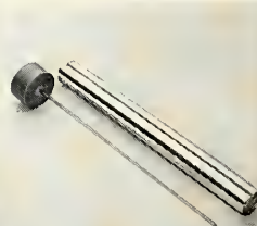
SEVEN INCH LONG, .078" DIAMETER, HOLE ELECTROLYTICALLY "DRILLED" IN UDIMET 700. ROD HAS BEEN SURFACE GROUND TO EXAMINE STRAIGHTNESS OF HOLE. NO WEAR ON ELECTRODE.
