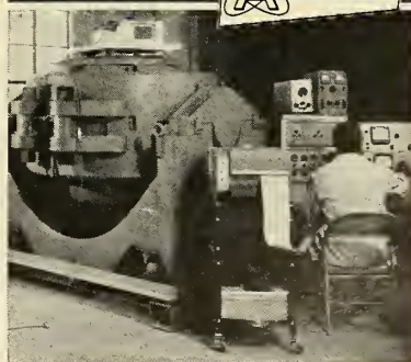
Test being conducted on the 12,500 force pound Vibration Machine. Accelerometer outputs are being automatically recorded for inclusion in the test report.
