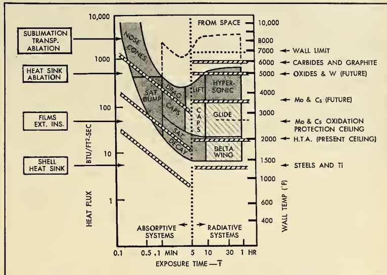
OVERALL CORRELATION of environmental conditions, re-entry vehicles, and thermostructural materials in the concept of re-entry.
