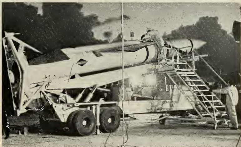
MOBILE BOMARC on transporter-erector is shown in this exclusive photo. Company feels this system will make the anti-aircraft bird more flexible, less vulnerable.
