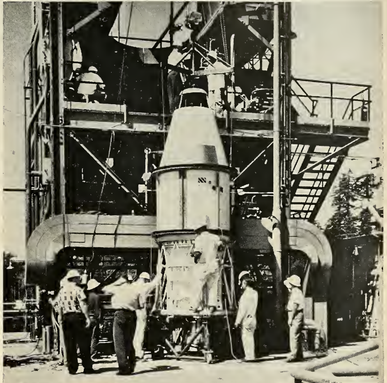
SECOND-STAGE Agena carried re-entry vehicle into polar orbit. After stabilization and proper attitude orientation, nose cone is separated and returns to earth.
