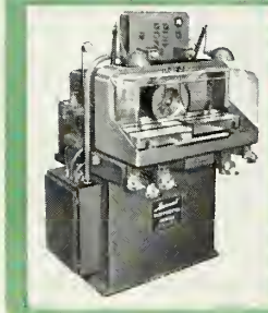
MACHINING POCKETS IN FRAGILE STAINLESS STEEL HONEY-COMB FREE OF LAYOVER AND BURR. PHOTO COURTESY EKSTROM, CARLSON & CO.
