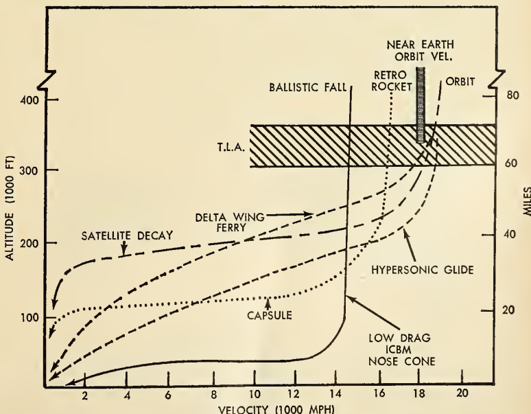
CHARACTERISTICS OF the various flight paths of re-entry vehicles. Flight path and vehicle form details determine actual aerodynamic heating.
