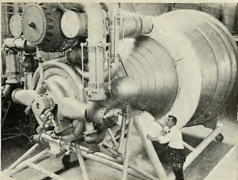
GIANT LIQUID rocket under development at Rocketdyne will provide 1½ million lbs. thrust in single cell for NASA's Nova vehicle.
