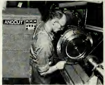
MOUNTING STATOR RING FOR ELECTROLYTIC MACHINING OF VANE TIPS TO ACHIEVE PRECISE CONCENTRICITY AND SIZE. OPERATION IS FAST AND ELIMINATES DEBURRING, SAVING LABOR COSTS AND REDUCING SCRAP.
