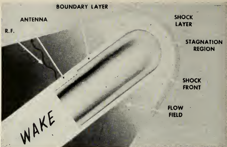
SHOCK EFFECT produced by a body traveling through the atmosphere at supersonic speeds. Much of the heat never reaches the surface of the vehicle.
