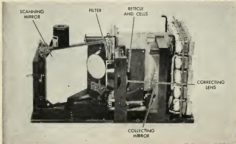
AVION's CODES IR detection system (cover removed) reportedly has 10 times the sensitivity of other search systems.
