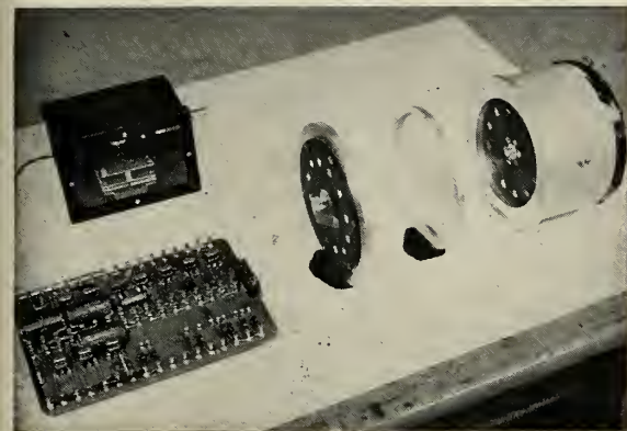
FIG. 2 —(at left) Exploded view of ultrasensitive microbarometer which could be used to measure pressure pulses from atomic bursts in space. Black box contains Decker Corp.'s T-42 transducer (Courtesy Prof. W. Kasner).
