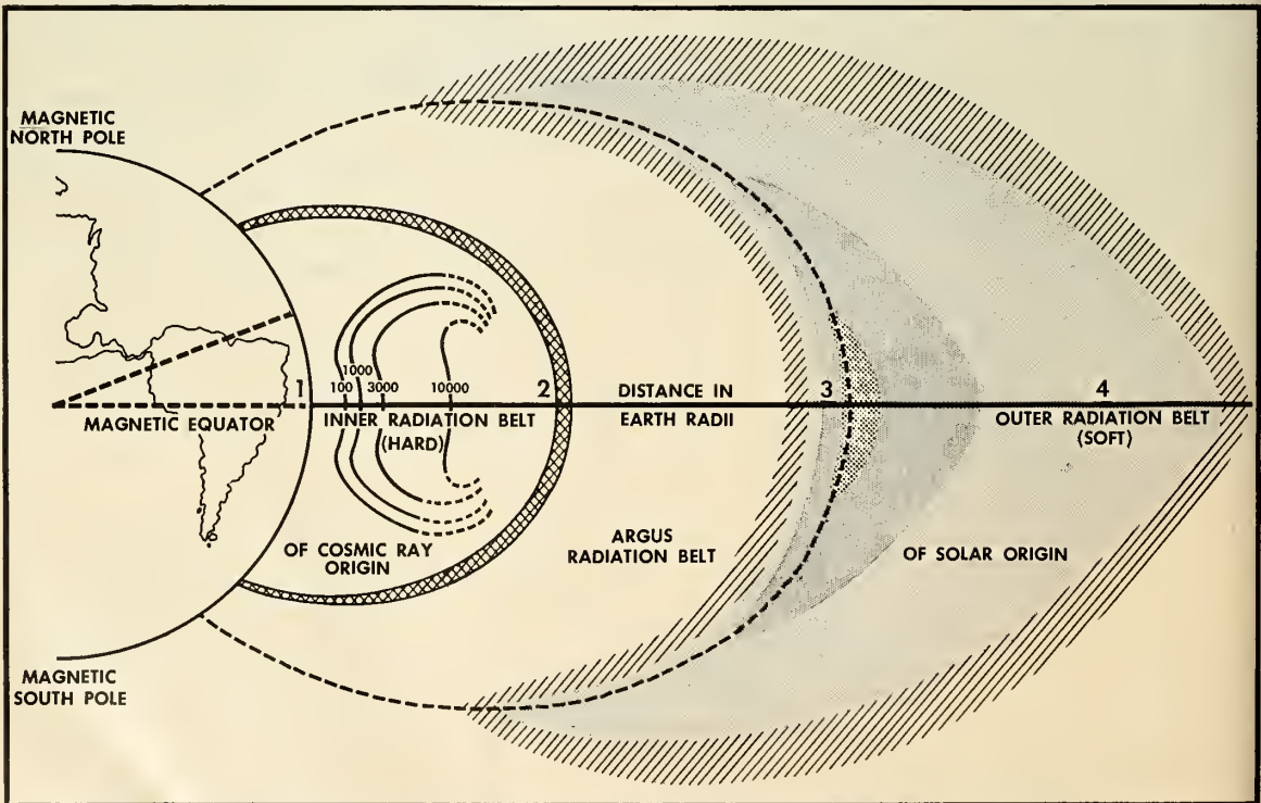
FIG. 1—Radiation belt intensities calculated from theory. For the inner belt, consisting mainly of hard (penetrating) protons, actual counting rates can be calculated. For the outer belt, made up largely of soft (easily shielded) electrons and protons, relative intensity distribution is calculated; the actual intensities will change, as will the position of the belt, depending on the amounts of fast plasma shot out from the sun. Location of Argus radiation is shown along the line of force reaching out to two earth radii (8000 miles from center of earth, or 4000 miles above sea level).
