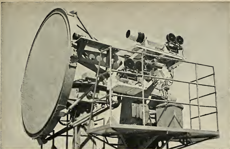
Mitchell Camera installation for radar tracking studies.
