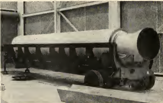
AEROJET-GENERAL will supply the solid fuel second stage for NASA's "all-purpose" Scout vehicle.
