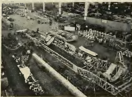
CRADLE FOR Atlas missile begins to take shape as I beams and cross braces are welded together.
