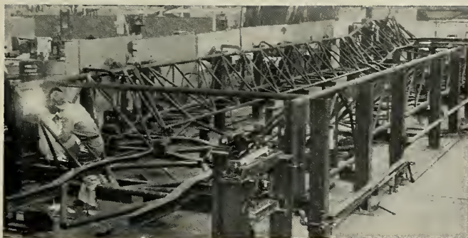
CRADLE FOR Atlas missile begins to take shape as I beams and cross braces are welded together.
