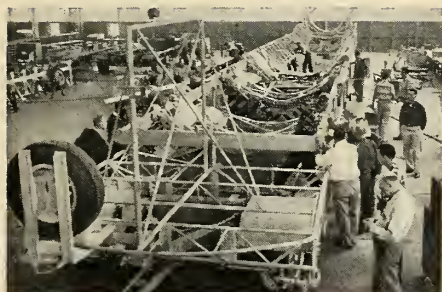
TECHNICIANS give final check to missile transport trailer and booster and nacelle carriage before taking out for road tests.
