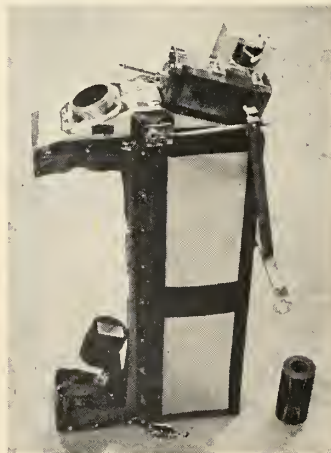
FIG. 4—Spectrograph designed to detect daytime aurora from a balloon. Half of the cover has been removed to show concave grating which is "blazed" to put most of light coming through slit (upper left) into red portion of the spectrum. Recording is done with specially sensitized film in cassette (upper right). Holder for filmstrips is shown next to spectrograph. Basic design of instrument follows that of Dr. R. Tousey, Naval Research Laboratory (Courtesy Profs. H. Griem and E. Hinnov).
